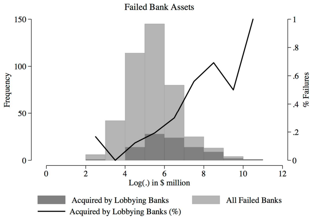
Figure 3: Histogram of Failed Bank Assets
