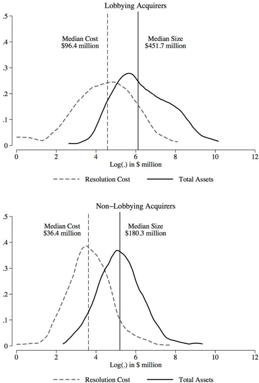
Figure 4: Kernel Density of Failed Bank Assets and Resolution Costs
