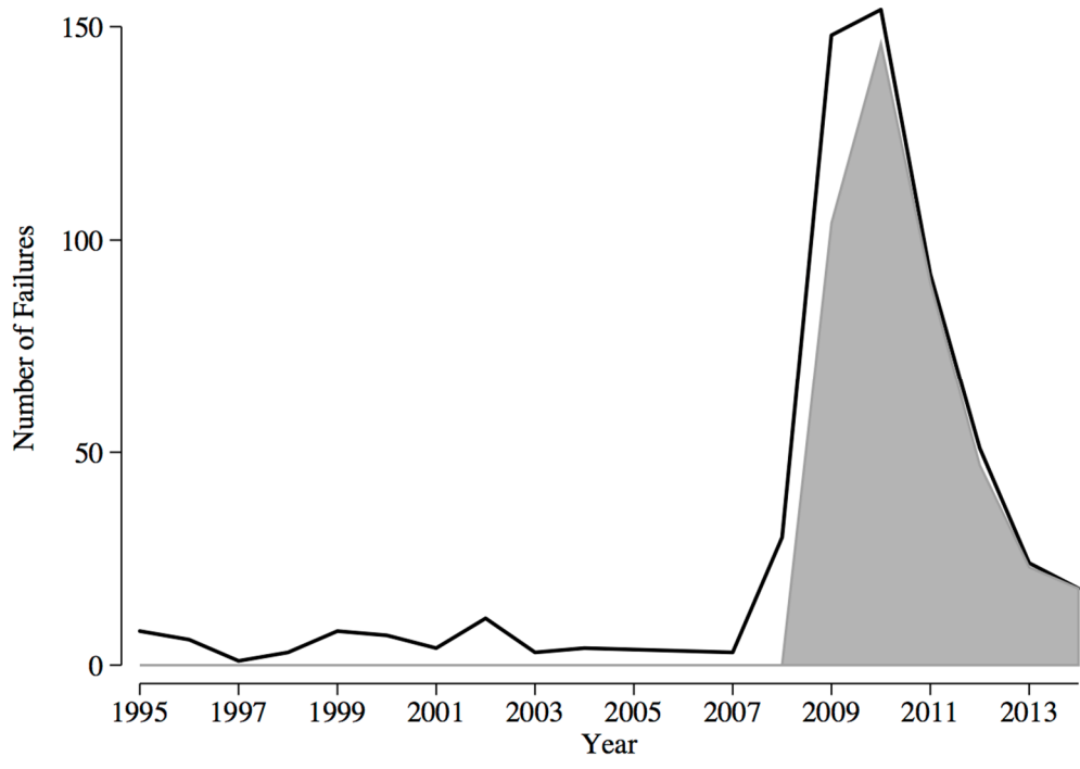
Figure 1: Number of Bank Failures
